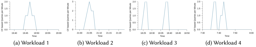
Fig. 4. Number of queries executed in CFs when evaluating the workloads
