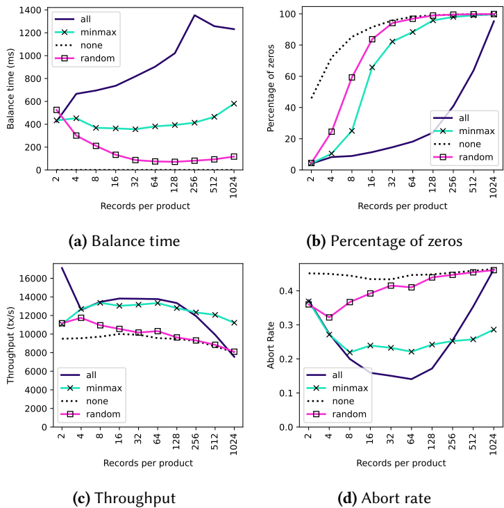
Fig. 14. Comparison between different balance algorithms.
