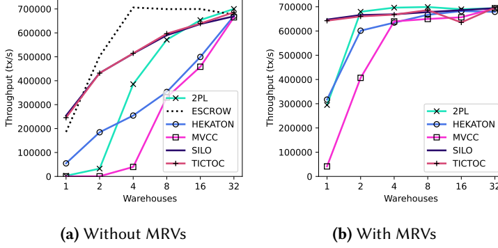
Fig. 11. Throughput comparison between different concurrency control techniques with and without MRVs. 2PL a) is equivalent to native of Figure 11; 2PL b) is equivalent to mrsv in Figure 11.
